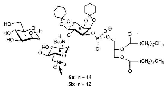
Scheme 2. Decisive intermediates
