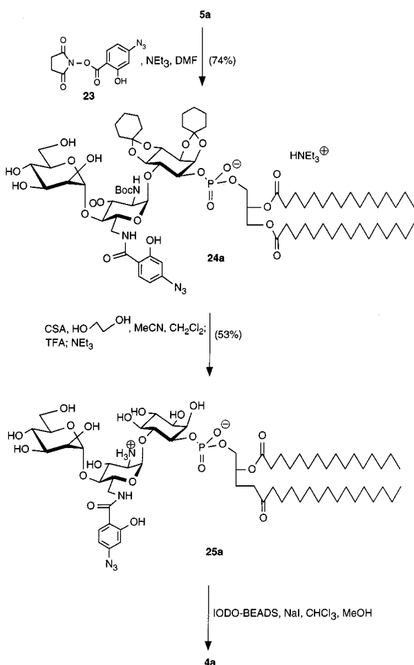
Scheme 6. Synthesis of 4a
