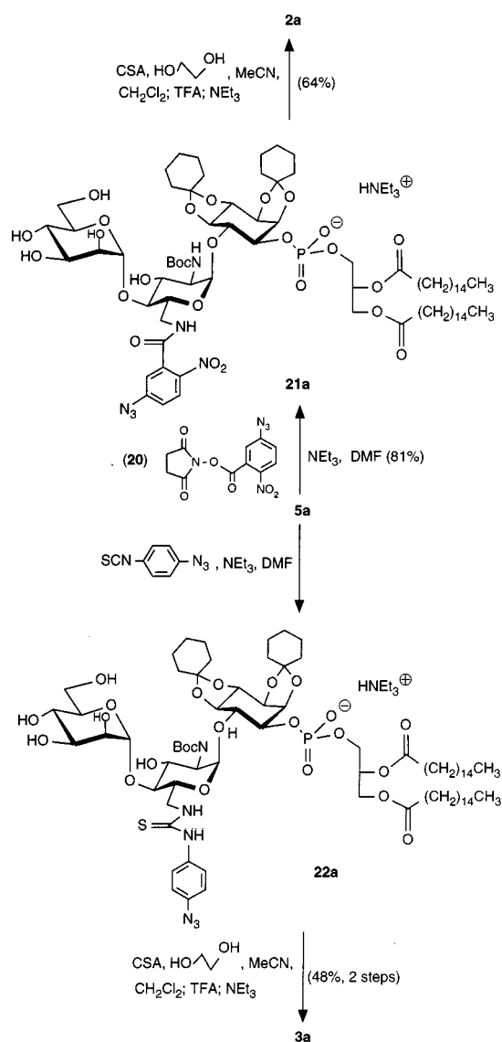
Scheme 5. Synthesis of 2a and 3a
