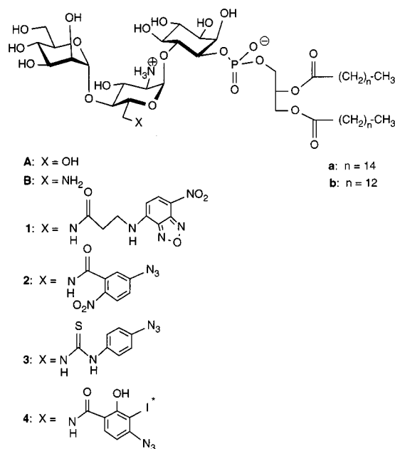
Scheme 1. Target molecules
