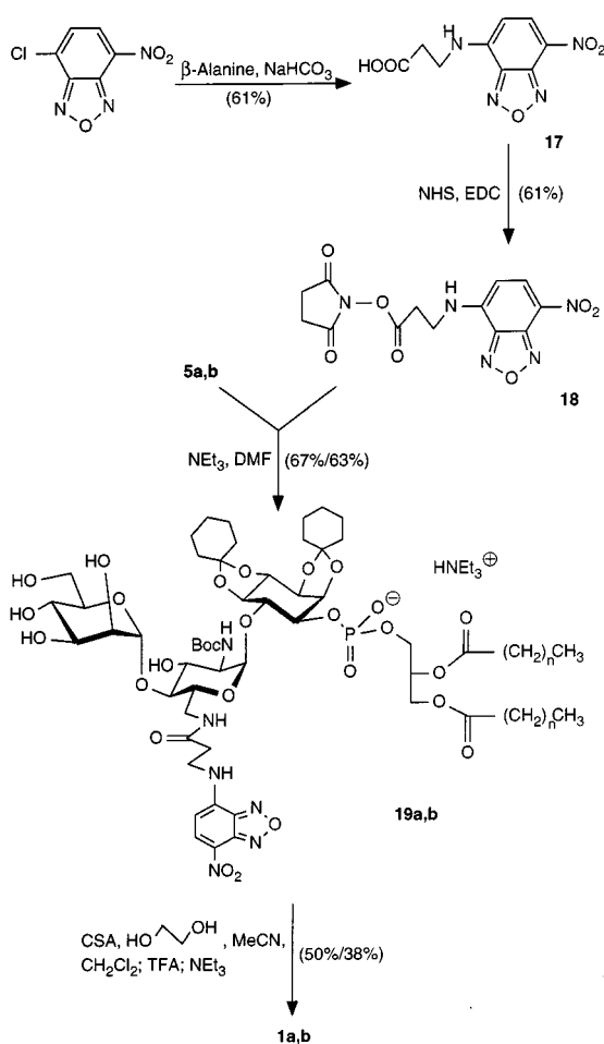
Scheme 4. Synthesis of 1a, b
