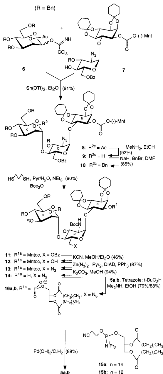
Scheme 3. Synthesis of 5a, b
